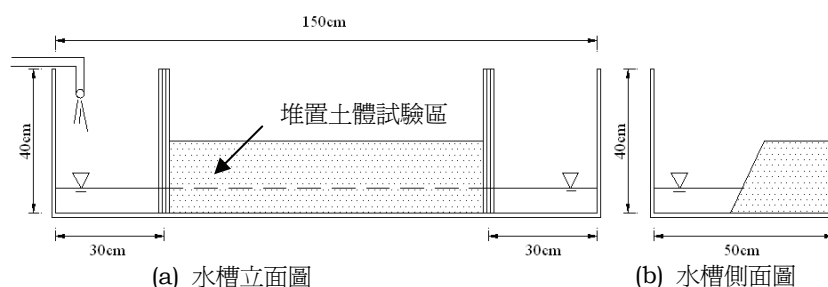
Fig.7 Schematic diagram of experimental flume
